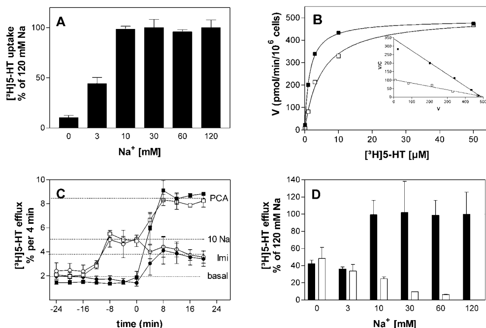
Fig. 5. Inward and outward transport of [ 3 H]5-HT under conditions of reduced extracellular sodium. A, HEK 293 cells stably expressing the hSERT were incubated in the presence of 100 \mu M [ 3 H]5-HT for 1 min in buffers containing different concentrations of Na + (Na + replaced by choline). For further experimental details, see legend to Fig. 1. Results are expressed as percentage of [ 3 H]5-HT uptake at 120 mM Na + and represent mean \pm S.E. ( n = 6 from three separate experiments). B, saturation analysis. Cells were incubated in the presence of different concentrations of [ 3 H]5-HT for 1 min in a buffer containing 120 mM Na + (■) or 10 mM Na + (□). For further experimental details, see legend to Fig. 1. Nonlinear fitting was used to calculate V_{max} and K_m . Inset displays Eadie-Hofstee plot of the same data. One of three experiments performed in duplicate is shown. C, superfusion experiment; cells were loaded with 5 \mu M [ 3 H]5-HT, superfused, and 4-min fractions collected. After three fractions (−16 min) the buffer was switched to a buffer containing 10 mM Na + (○, □; Na + replaced by choline) followed by the addition (0 min) of 10 \mu M PCA (□) or 10 \mu M imipramine (○). Controls (●, ■) received the same drugs but were not switched to 10 mM Na + . Dotted lines indicate mean fractional rates of efflux at the different experimental conditions. Symbols represent mean \pm S.E. ( n = 9 from three separate experiments). D, superfusion experiments as described in C were performed at different concentrations of extracellular Na + . Open columns represent efflux induced by low Na + , and closed columns represent efflux in the presence of low Na + plus PCA. All PCA effects were corrected for the efflux induced by imipramine at the corresponding buffer condition. All data are presented as percentage of the PCA effect at 120 mM Na + . Columns represent mean \pm S.E. ( n = 6 from two separate experiments). Experiments shown in B and C were performed on the same day. Cells for all experiments, 6 weeks in culture.
