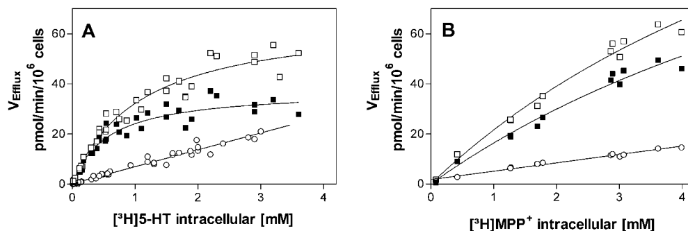
Fig. 4. Relationship between intracellular substrate concentration and PCA-induced efflux. HEK 293 cells stably expressing the hSERT were grown on 5-mm coverslips, preincubated with different concentrations of [ 3 H]5-HT (0.15–10 \mu\text{M} ) or [ 3 H]MPP + (2–128 \mu\text{M} ), superfused, challenged with 10 \mu\text{M} PCA, and V_{efflux} values determined as explained in Fig. 3. In cells preincubated with [ 3 H]5-HT V_{efflux} values for 10 \mu\text{M} imipramine were also determined in parallel superfusion. Intracellular substrate concentrations at the time of drug addition were calculated from the sum of radioactivity remaining in the cells at the end of the experiment and the superfusate fractions. The calculation was based on a cell volume of 1.25 pL/cell and a cell number of 27,000 cells/coverslip (under Materials and Methods ). A, [ 3 H]5-HT experiments; V_{efflux} values for PCA (■) were calculated from total PCA-induced efflux (□) minus diffusion-based efflux estimated from the linear regression line of the V_{efflux} values for imipramine (○). Nonlinear fitting was used to calculate the maximal efflux rate ( V_{max} for reverse transport; 38 pmol/min/10 6 cells) and that intracellular concentration of [ 3 H]5-HT at which the half-maximal rate of reverse transport was reached ( K_m for reverse transport; 564 \mu\text{M} ; see also text). For each drug, n = 30 ; one data point is one superfusion chamber. B, [ 3 H]MPP + experiments; V_{efflux} values for PCA (■) were calculated from total PCA-induced efflux (□) basal efflux during the first 16 min before the addition of PCA (○). Nonlinear fitting was performed as in A. For calculated parameters ( V_{max} and K_m for reverse transport), see text ( n = 12 ; one data point is one superfusion chamber). Cells for experiments in A, 4 weeks in culture; cells for experiments in B, 14 weeks in culture.
