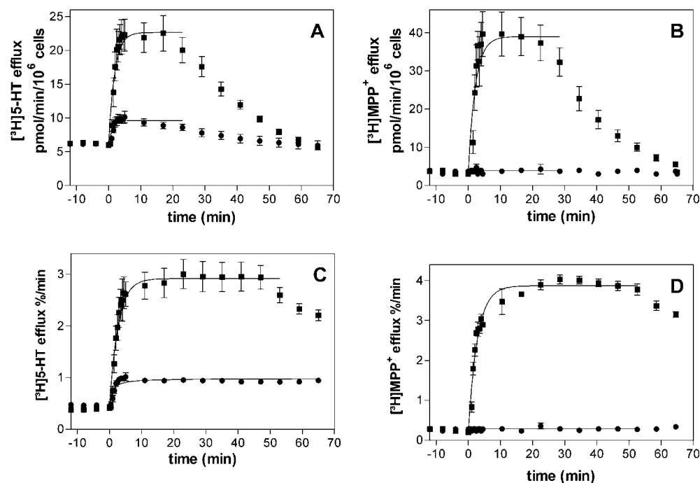
Fig. 3. Determination of outward transport rates ( V_{\text{efflux}} ). HEK 293 cells stably expressing the hSERT (4–5 weeks in culture) were grown on 5-mm coverslips, preincubated with [ ^3\text{H} ]5-HT (5 \mu\text{M} ; A and C) or [ ^3\text{H} ]MPP ^+ (64 \mu\text{M} ; B and D) and superfused. After a 45-min washout period four 4-min fractions of basal efflux were collected. Then the buffer was switched to a buffer containing 10 \mu\text{M} PCA (■) or 10 \mu\text{M} imipramine (●), and ten 30-s fractions followed by ten 6-min fractions were collected. A and B, data are expressed as pmol/min/ 10^6 cells calculated with a number of 27,000 cells/coverslip (under Materials and Methods ). C and D, data of A and B, respectively, are shown as fractional rates; i.e., the radioactivity in each superfusate fraction was expressed as percentage of the activity in the cells at the beginning of that fraction. Efflux rates ( V_{\text{efflux}} ) were estimated using nonlinear fitting of the individual data points from 0 min (time of drug addition) to 15 min (A and B) or 0 to 45 min (C and D). The mean value of the four baseline fractions was used for correction and subtracted from each data point before the fitting procedure was performed. Symbols represent mean \pm S.E. ( n = 8 –12, from at least two separate experiments; one observation is one superfusion chamber).
