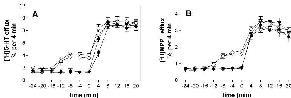
Fig. 8. [ ^3\text{H} ]5-HT and [ ^3\text{H} ]MPP ^+ efflux induced by 5-HT and MPP ^+ under standard and low-sodium conditions. HEK 293 cells stably expressing the hSERT were loaded with 5 \mu\text{M} [ ^3\text{H} ]5-HT (A, cells 5 weeks in culture) or 64 \mu\text{M} [ ^3\text{H} ]MPP ^+ (B, cells 3.5 weeks in culture), superfused, and 4-min fractions collected. After three fractions (–16 min) the buffer was switched to a buffer containing 10 mM \text{Na}^+ ( \text{Na}^+ replaced by choline) followed by the addition (0 min) of 10 \mu\text{M} 5-HT (◇) or 1 mM MPP ^+ (▽). Controls (▼, ◆) received the same drugs but were not switched to 10 mM \text{Na}^+ .
