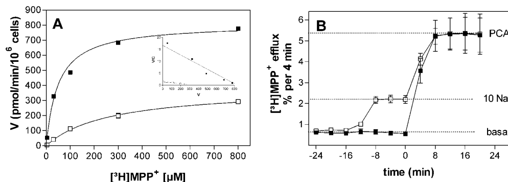
Fig. 6. Inward and outward transport of [ 3 H]MPP + under conditions of reduced extracellular sodium. A, HEK 293 cells stably expressing the hSERT were incubated in the presence of different concentrations of [ 3 H]MPP + for 1 min in a buffer containing 120 mM Na + (■) or 10 mM Na + (□). For further experimental details, see legend to Fig. 1. Nonlinear fitting was used to calculate V_{max} and K_m . Inset displays Eadie-Hofstee plot of the same data. One of three experiments performed in duplicate is shown. B, time course of superfusion experiments; cells were loaded with 64 \mu M [ 3 H]MPP + , superfused, and 4-min fractions collected. After three fractions (−16 min) the buffer was switched to a buffer containing 10 mM Na + (□; Na + replaced by choline) followed by the addition (0 min) of 10 \mu M PCA (□). Controls (■) also received PCA but were not switched to 10 mM Na + . Dotted lines indicate mean fractional rates of efflux at the different experimental conditions. Symbols represent mean \pm S.E. ( n = 9 from three separate experiments). Experiments shown in A and B were performed on the same day. Cells for all experiments, 5 weeks in culture.
