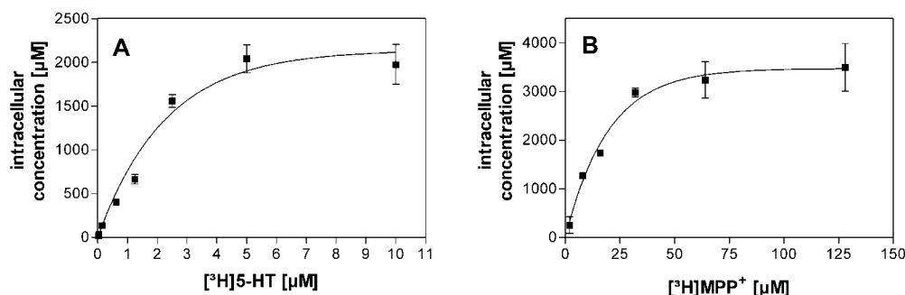
Fig. 2. Intracellular retention of [ ^3\text{H} ]5-HT and [ ^3\text{H} ]MPP ^+ in superfusion experiments. HEK 293 cells stably expressing the hSERT were grown on 5-mm glass coverslips, preincubated with various concentrations of [ ^3\text{H} ]5-HT (A) or [ ^3\text{H} ]MPP ^+ (B), transferred to superfusion chambers, and superfused for 45 min at room temperature. The cells were then lysed, and the retained radioactivity determined and used for the calculation of intracellular concentrations. As outlined under Materials and Methods , the calculation was based on a cell volume of 1.25 pL/cell and a cell number of 27,000 cells/coverslip. Symbols represent mean \pm S.E. ( n = 8 –16 from at least two separate experiments; one observation is one superfusion chamber). Data were fitted using nonlinear regression analysis. Cells for experiments in A, 3.5 weeks in culture; cells for experiments in B, 12 weeks in culture.
