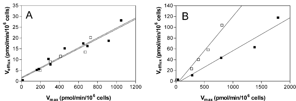
Fig. 7. Relationship between maximal rates of inward and outward transport of [ ^3\text{H} ]5-HT and [ ^3\text{H} ]MPP ^+ under control conditions and under conditions of reduced extracellular sodium. Batches of cells that had been kept in culture for different periods of time (3.5–12 weeks) were used for uptake and superfusion experiments performed in parallel under standard conditions (■, 120 mM \text{Na}^+ ) and low- \text{Na}^+ conditions (□, 10 mM; \text{Na}^+ replaced by choline). V_{\text{max}} values for the uptake of [ ^3\text{H} ]5-HT and [ ^3\text{H} ]MPP ^+ were determined using saturation analyses as described in legends to Figs. 5B and 6A, respectively. V_{\text{efflux}} values were determined in superfused cells preincubated with 5 \mu\text{M} [ ^3\text{H} ]5-HT or 64 \mu\text{M} [ ^3\text{H} ]MPP ^+ and challenged with 10 \mu\text{M} PCA. For experimental details, see legend to Fig. 3. A, [ ^3\text{H} ]5-HT experiments; B, [ ^3\text{H} ]MPP ^+ experiments. For correlation coefficients see text.
