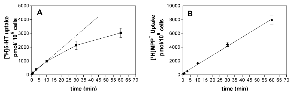
Fig. 1. Time course of [ ^3\text{H} ]5-HT and [ ^3\text{H} ]MPP ^+ uptake in HEK 293 cells stably expressing the hSERT. HEK 293 cells stably expressing the hSERT were distributed in 24-well plates as described under Materials and Methods ( 5 \times 10^4 cells) and incubated in the presence of 2.5 \mu\text{M} [ ^3\text{H} ]5-HT (A) or 75 \mu\text{M} [ ^3\text{H} ]MPP ^+ (B) for different periods of time, washed, solubilized, and the tritium activity was determined by liquid scintillation counting. Nonspecific uptake was defined as uptake in the presence of 30 \mu\text{M} clomipramine. Symbols represent mean \pm S.E. ( n = 6 from three separate experiments). Linear regression analysis was performed using the data points from 0 to 10 min in A (broken line) and all data points in B. Cells for experiments in A, 11 weeks in culture; cells for experiments in B, 7 weeks in culture.
